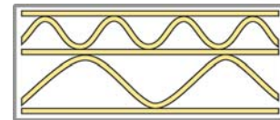
Custom Double Wall Corrugated Design 310 mil Thick
