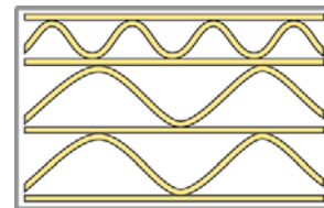
Custom Triple Wall Corrugated Design 650 mil Thick
